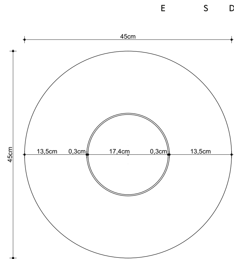
CUBA BRUMA 1:5
